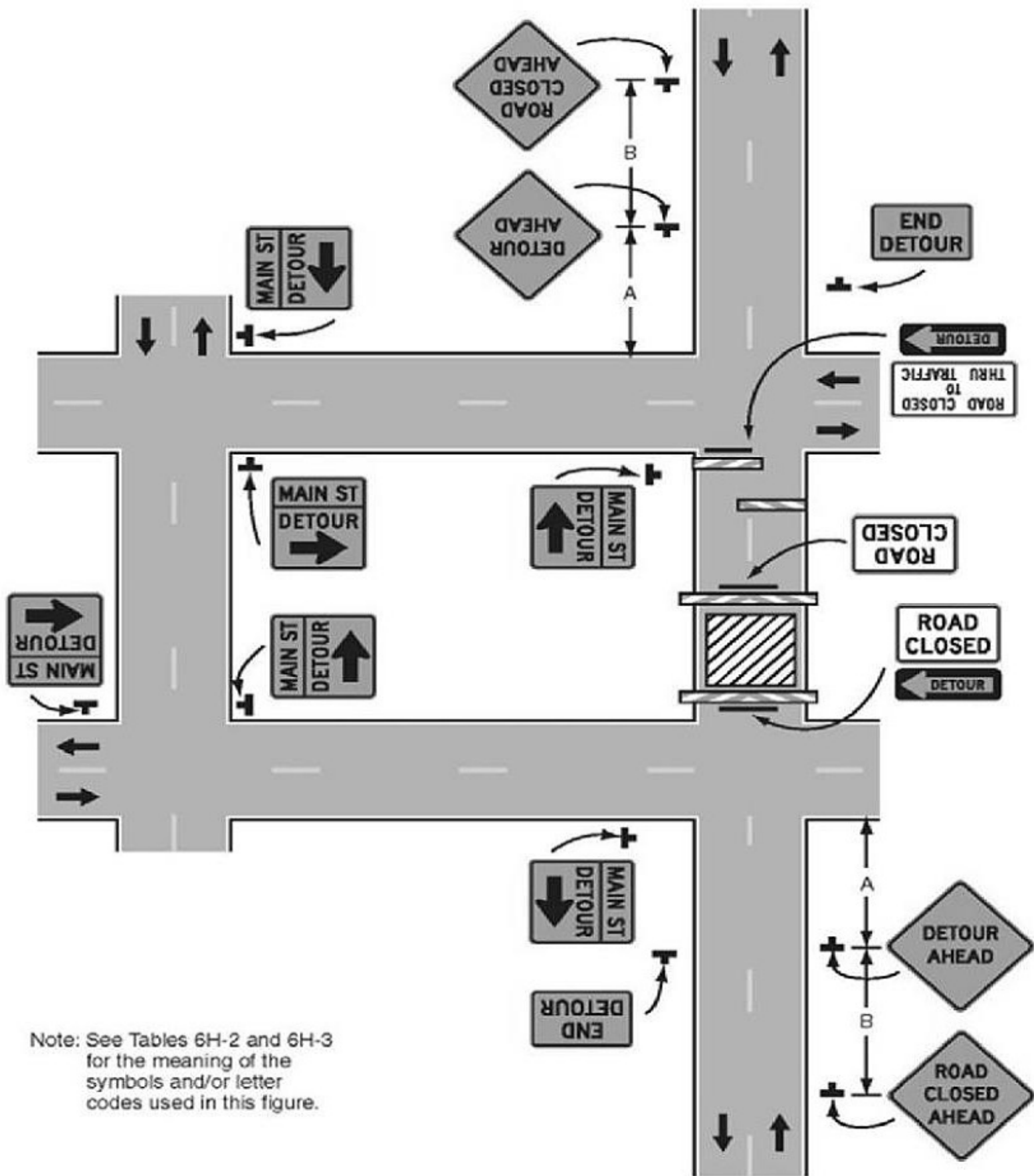
Typical Application 20
