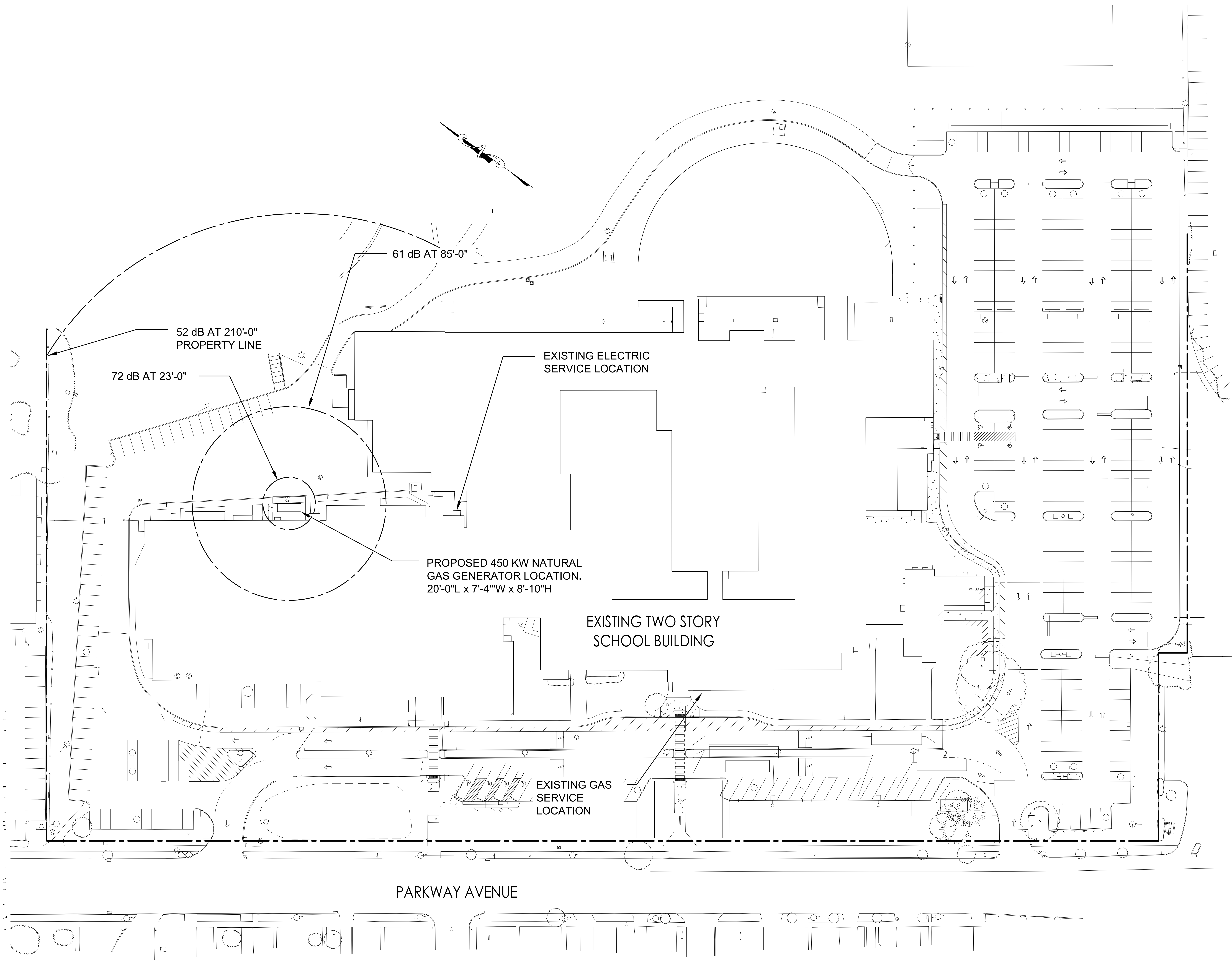
SITE PLAN SCALE: 1" = 30'-0"
