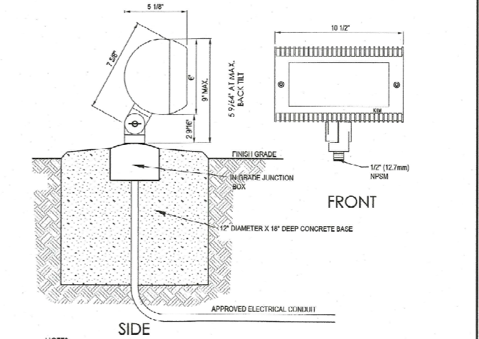
Monument Sign Light Detail:
